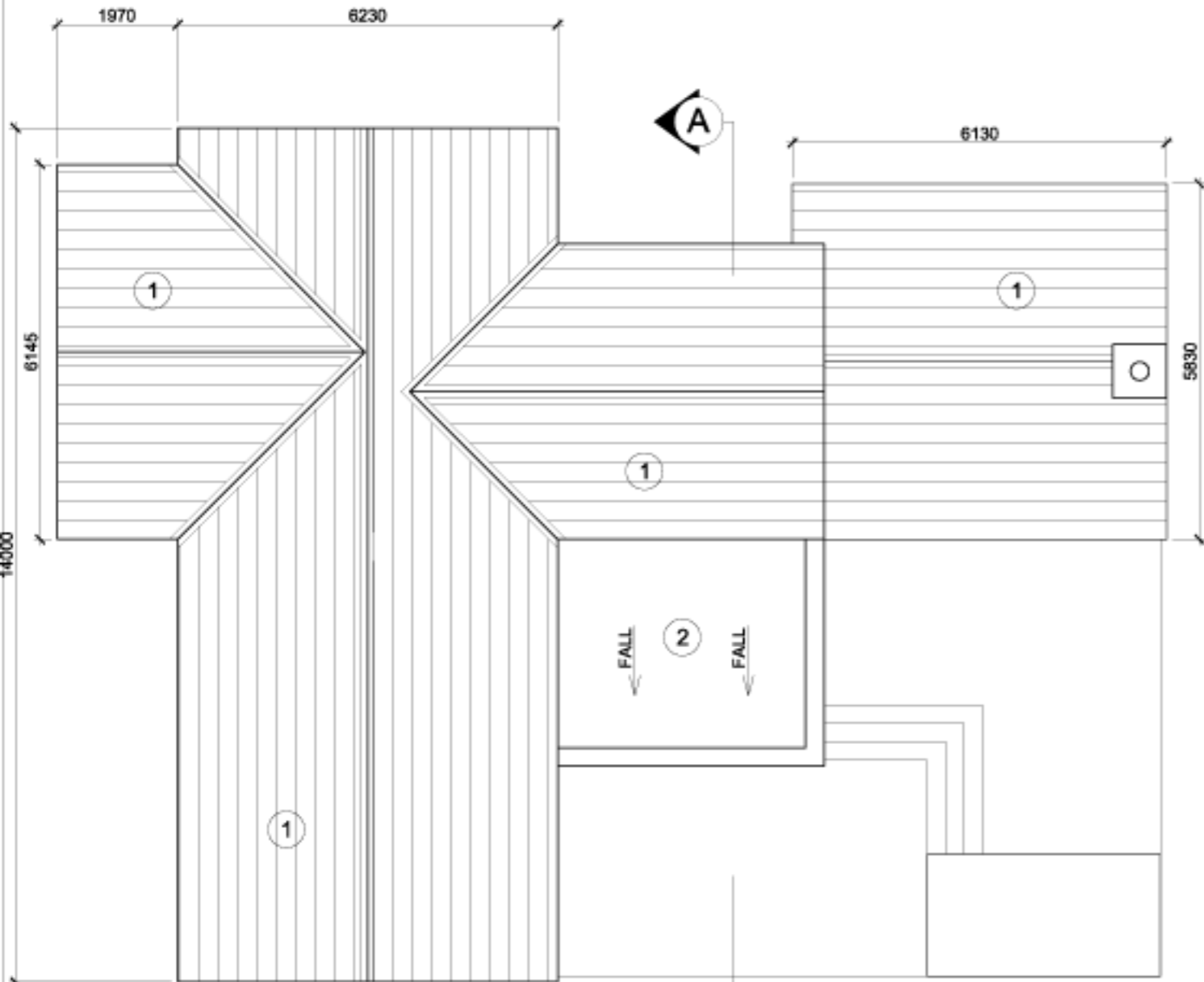
01 ROOF PLAN TYPE 2 1:100 @ A3
